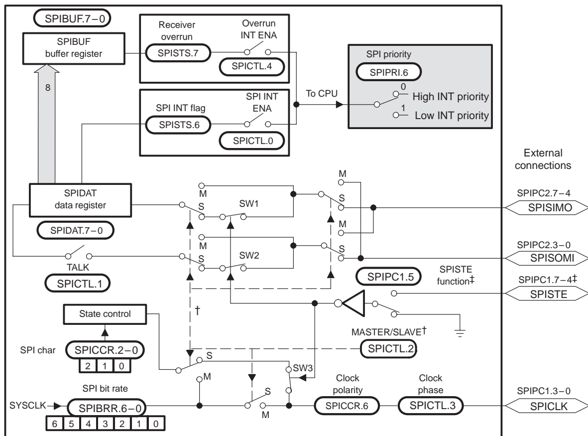
Figure 9–1. 4-Pin SPI Module Block Diagram (Slave Mode)
