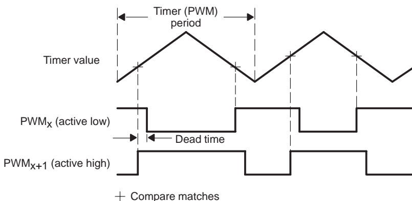
Figure 6–22. Symmetric PWM Waveform Generation With Full Compare Units and PWM Circuits ( x = 1, 3, \text{ or } 5 )
